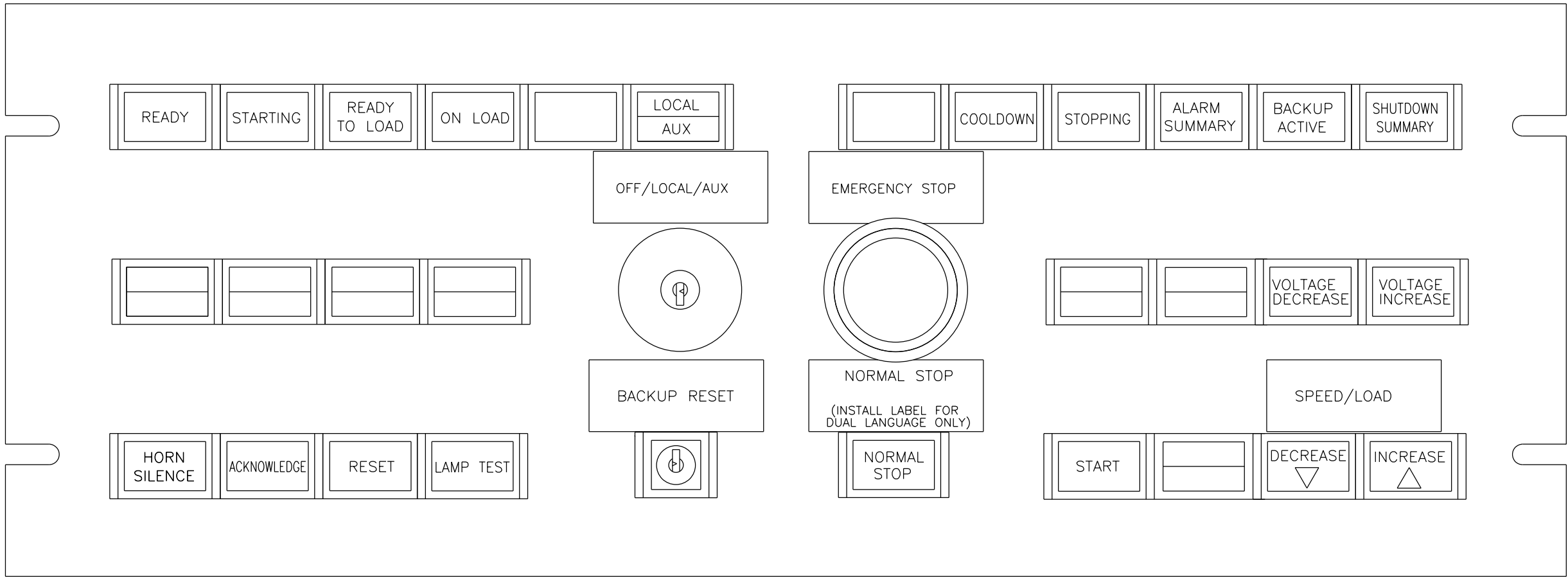
FRONT VIEW
